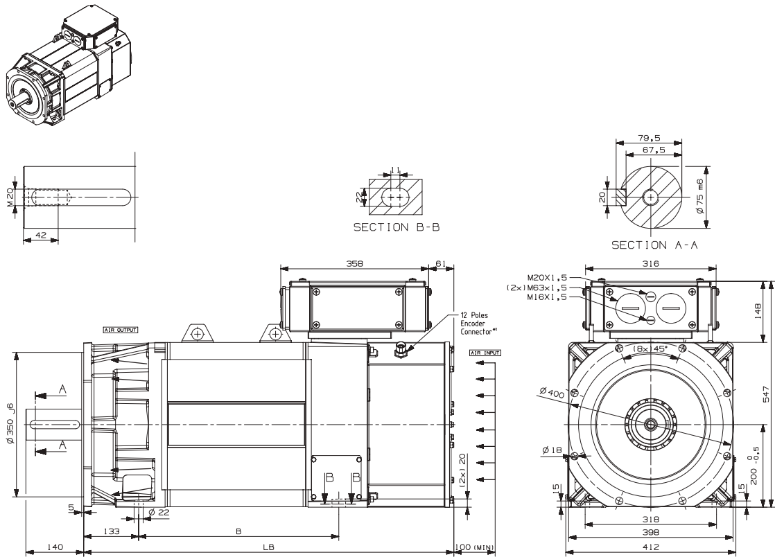
Motor types, IP54, H200
