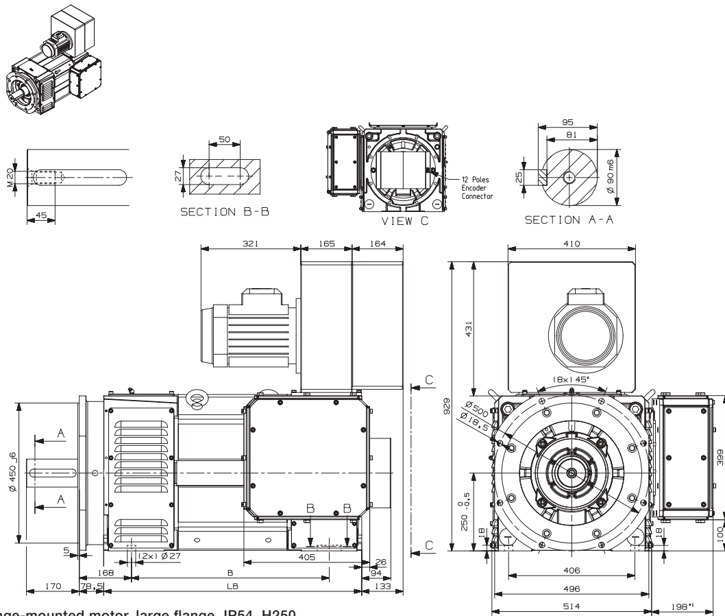
Motor types, flange-mounted motor, large flange, IP54, H250
