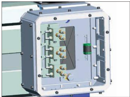
Fig. 6. Terminal board for motor sizes 250.
