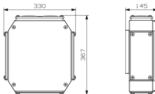
Fig. 3. Motor size 200, standard design with 6 terminals
