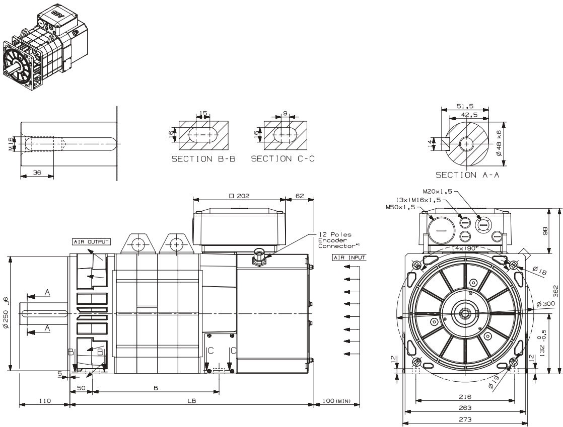
Motor types, IP54, H132
