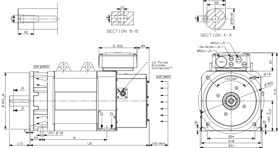
Motor types, IP54, H160
