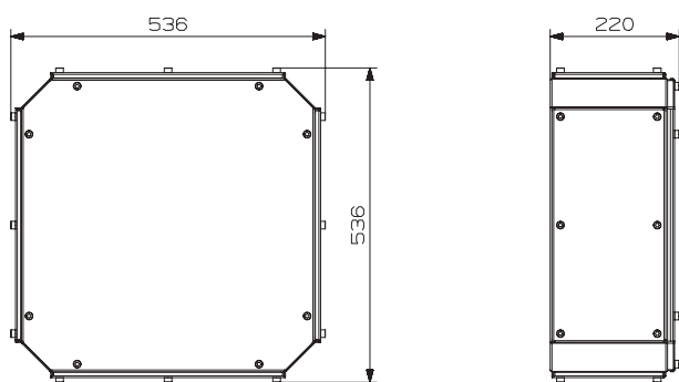
Fig. 4 Motor size 250, with larger than standard terminal box (variant code 019), with 21 terminals
